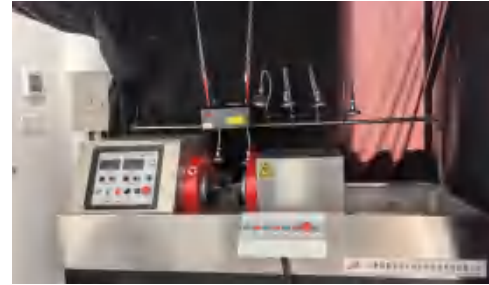
Magnetic particle flaw detector 磁粉探伤机
