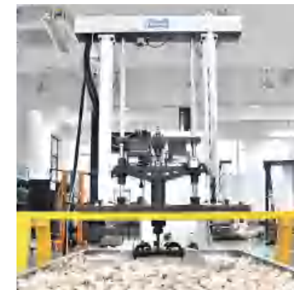
Drop Hammer Impact Test System 落锤冲击试验系统
