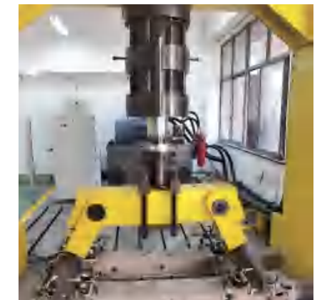
Electro-Hydraulic Servo Rail Clip Fatigue Testing Machine (100T) 电液伺服弹条疲劳试验机 (100T)
