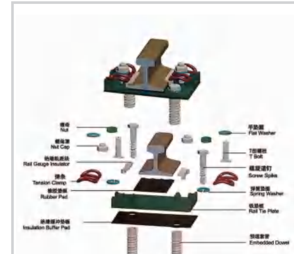
DJK5-1 Fastening System DJK5-1 型扣件系统
