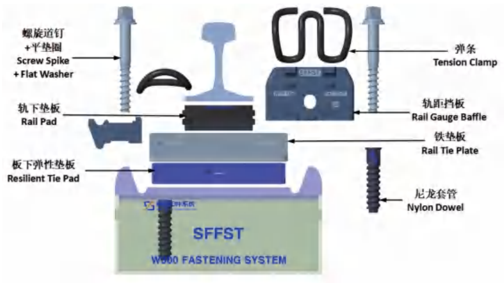
Components of single sleeper 单根轨枕扣件各零部件配置表
