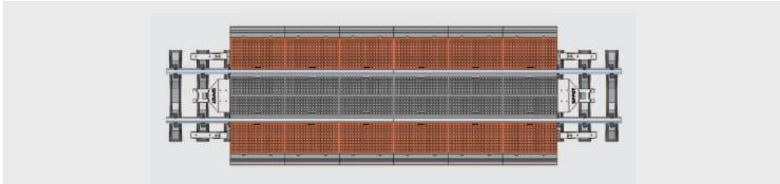
Rubber Level Crossing Panel_ Standard Gauge 橡胶道口铺面板_标轨
