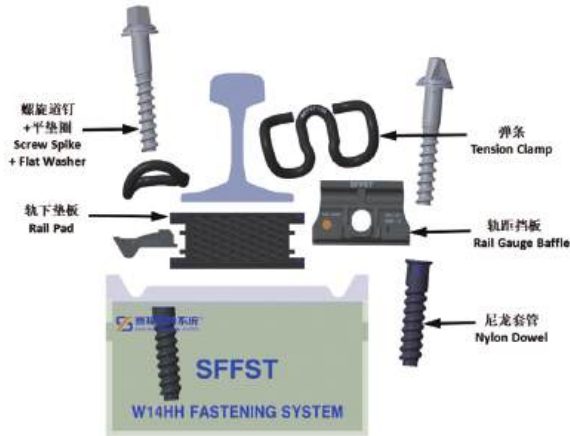
W14HH Fastening System
