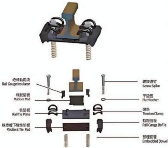
WJ-8 Fastening System
