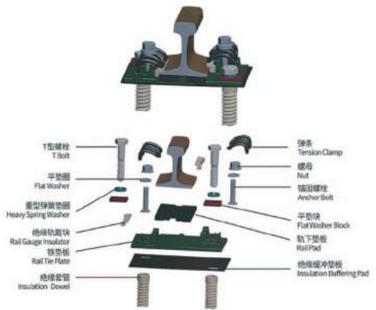
WJ-2A Fastening System
